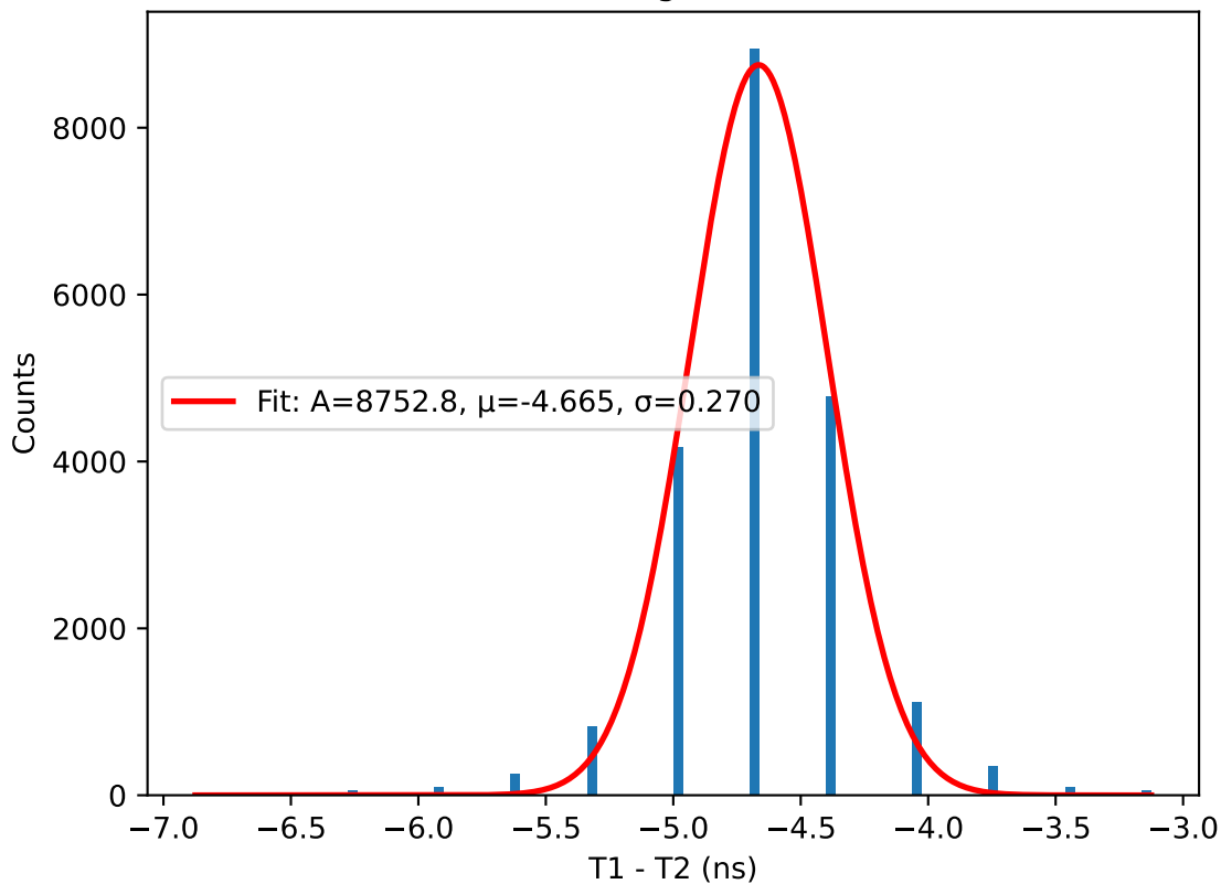
T1 - T2 histogram for 45.0V
