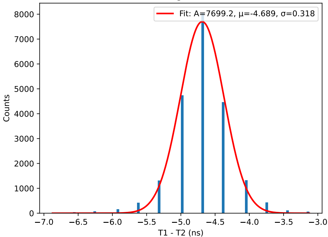
T1 - T2 histogram for 43.0V
