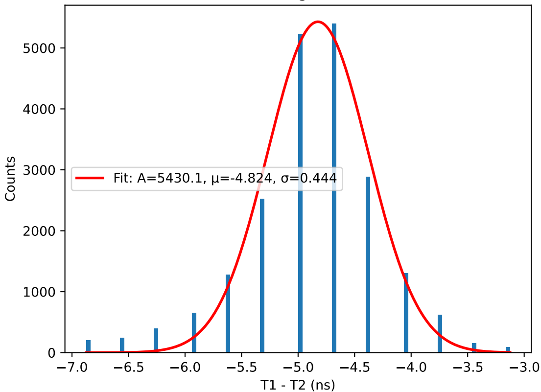
T1 - T2 histogram for 41V
