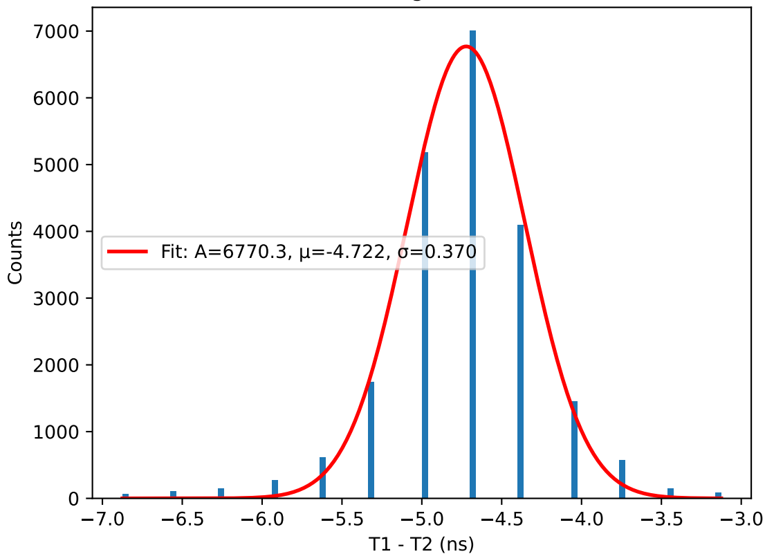
T1 - T2 histogram for 42.0V
