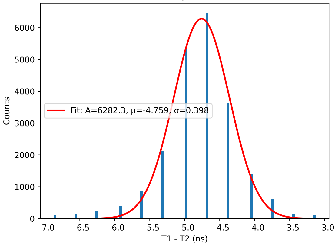
T1 - T2 histogram for 41.5V
