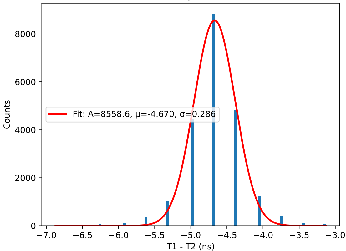
T1 - T2 histogram for 44.0V
