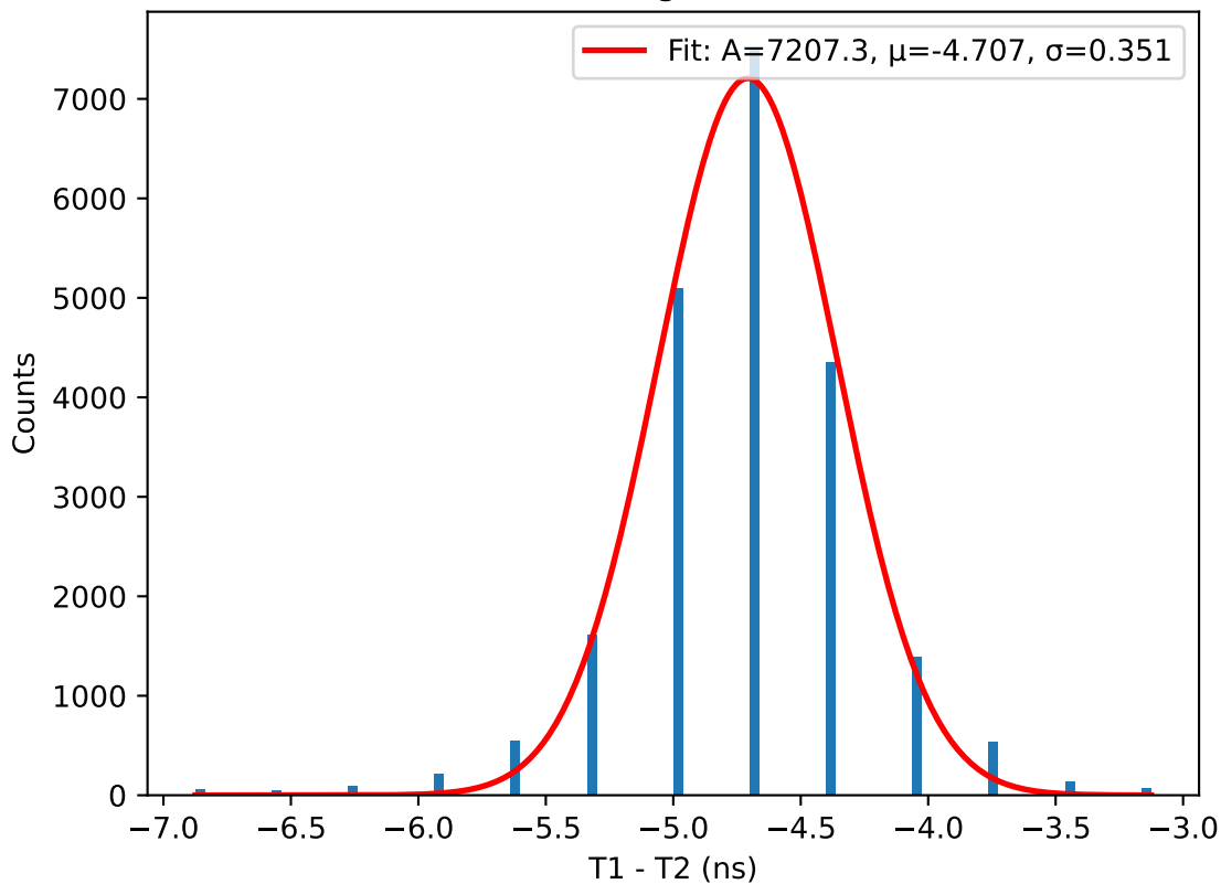
T1 - T2 histogram for 42.5V
