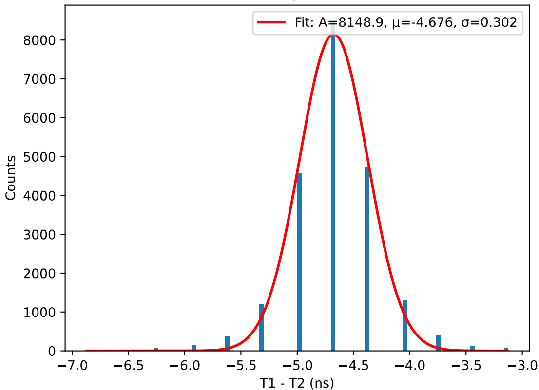
T1 - T2 histogram for 43.5V
